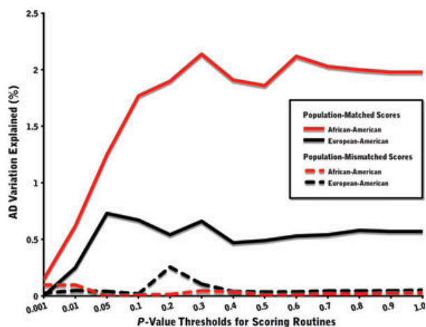
Figure 1: Variance in AD explained by genome-wide scores for AA and EA subjects. Polymarker scoring routines based on AD status were designed for thirteen GWAS significance thresholds (plotted against the x-axis) using COGA data and applied to SAGE target samples. The y-axis represents Nagelkerke's pseudo R^2 , the amount of variation in AD accounted by the SAGE scores, computed for routines that are both population-matched and mismatched across the COGA and SAGE data sets.
