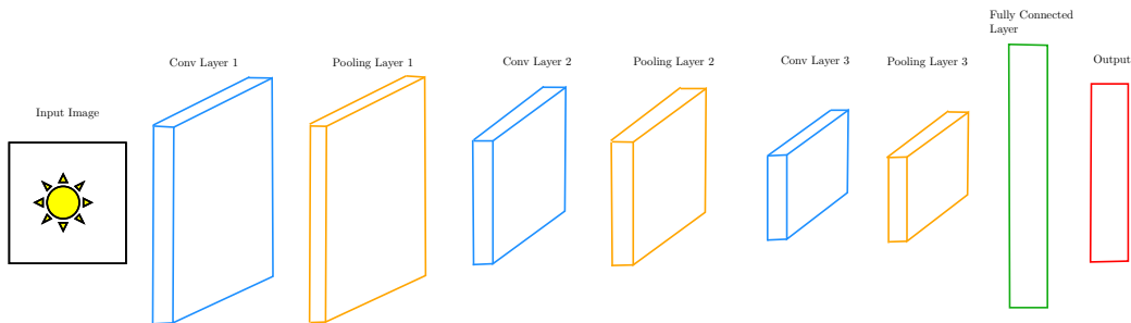
Figure 2.7: Example of CNN architecture.
