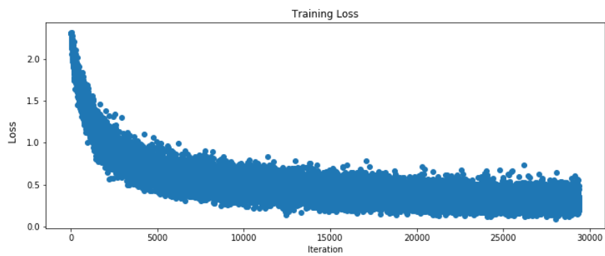
Figure 5.3: Training loss with Dropout.
