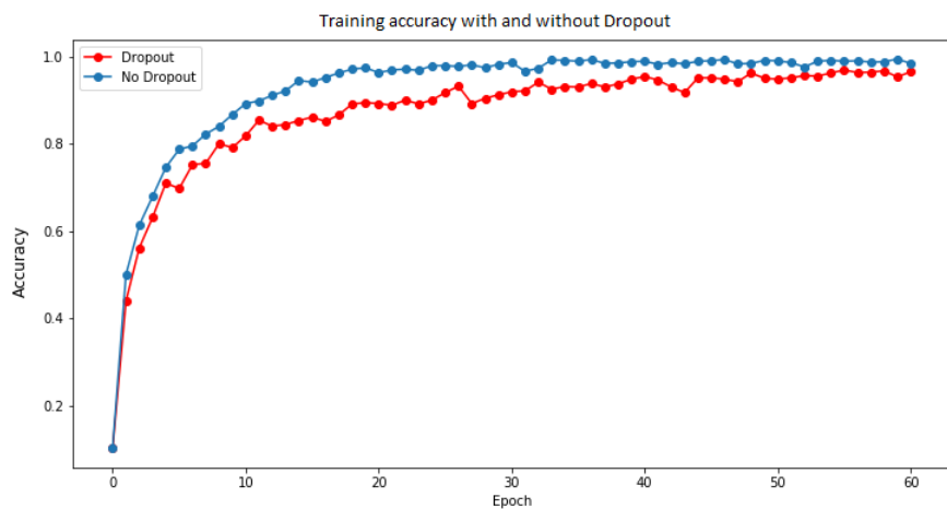
Figure 5.5: Training accuracy Comparison with and without Dropout.
