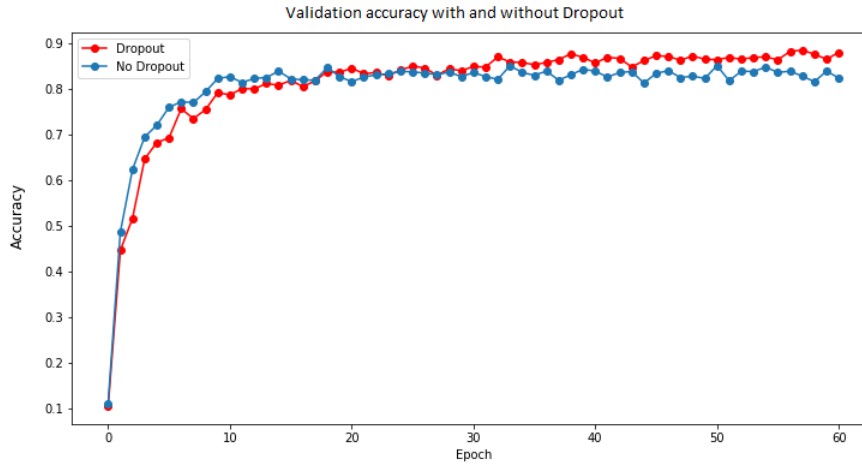
Figure 5.6: Validation accuracy Comparison with and without Dropout.
