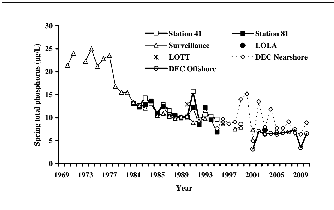
Figure 4b. Long-term spring (Apr – May) total phosphorus concentrations in Lake Ontario, 1970 - 2010. Data from 1970 – 2001 are from Environment Canada’s Surveillance Program. Station 41 and 81 are from the Department of Fisheries and Oceans Canada’s Bioindex Program. LOTT data is from the Lake Ontario Trophic Transfer Project. LOLA data is from the Lake Ontario Lower Food Web Assessment. Data from 1995 – 2010 are from the NYSDEC Biomonitoring Program.
