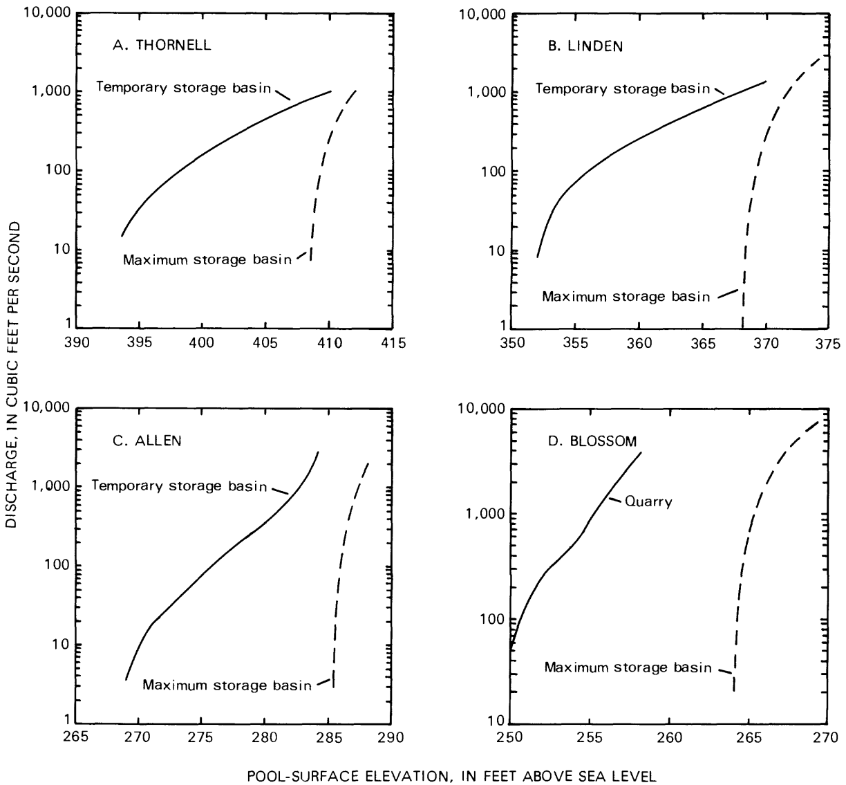
Figure 4.--Stage-vs-discharge relations for simulated temporary- and maximum-storage basins at each site. (Site locations are shown in fig. 1.)
