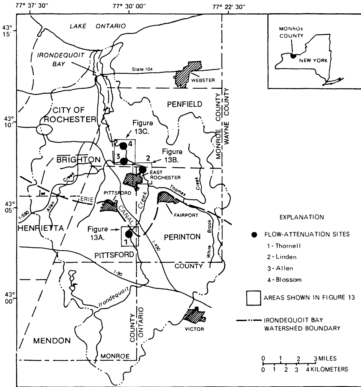
Figure 1.--Principal geographic features of Irondequoit Creek basin and locations of simulated flow-attenuation basins.
