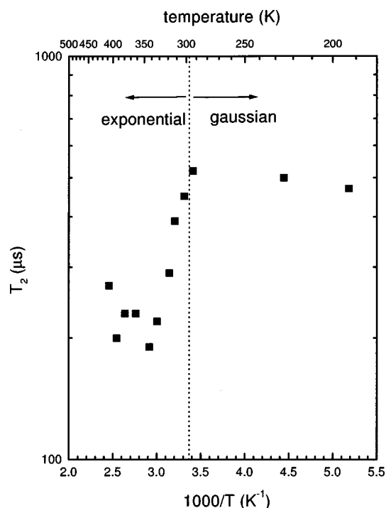
FIG. 3. T_2 measurements on the NIST sample. The measured T_2 represents the decay of the spin-echo envelope and thus is an average over the sites. Above 300 K, T_2 is shorter and describes an exponential decay. This suggests that motion-driven fluctuations in the quadrupole interaction control T_2 above 300 K.
