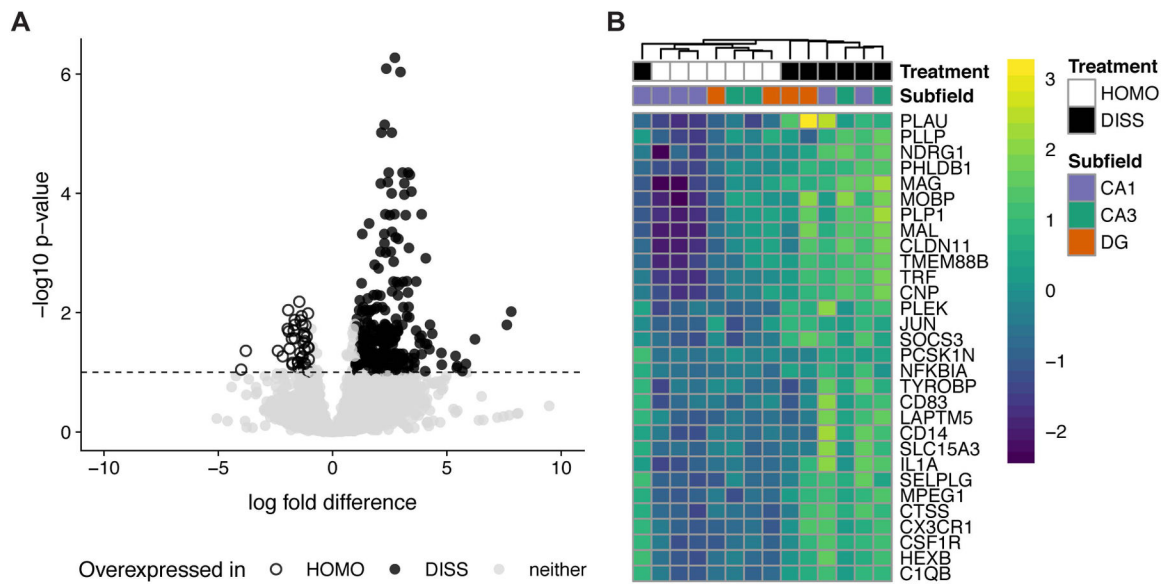
Figure 2. Enzymatic dissociation has a moderate effect on hippocampal gene expression patterns compared to homogenized tissue.
