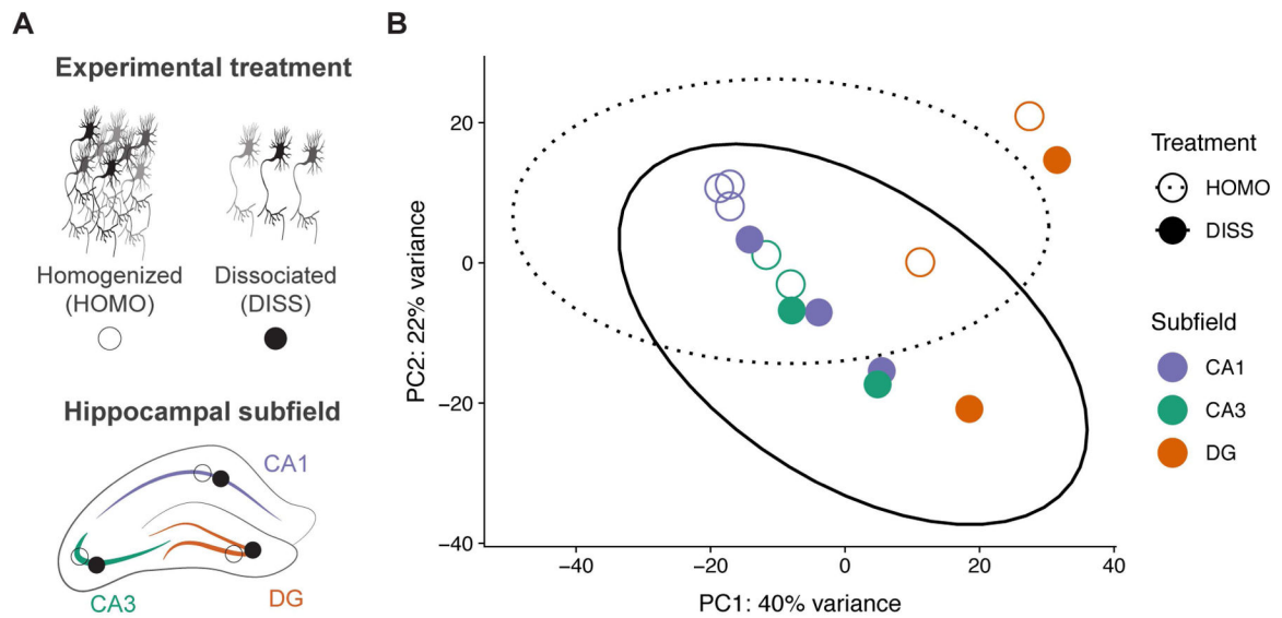
Figure 1. Experimental design and global expression gene expression patterns.
